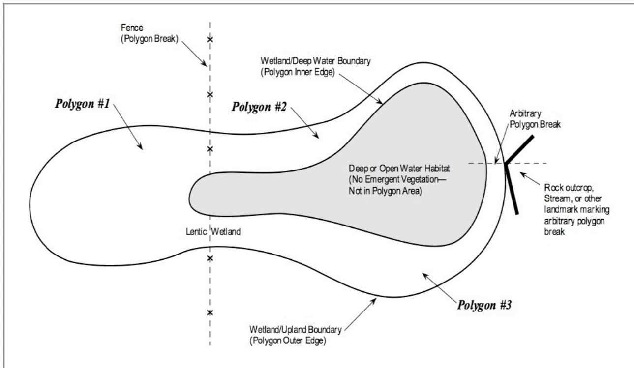
Figure 1. Schematic drawing of a lentic (still water) wetland showing: 1) delineation of polygons on larger systems, i.e. those too big to inventory as a single polygon (more than about 0.5 mi [1.6 km] in length) or those with managerial breaks crossing them; 2) a typical relationship between deep water habitat (lacking emergent vegetation) and surrounding lentic wetland, which includes all areas of persistent emergent vegetation in standing water.
